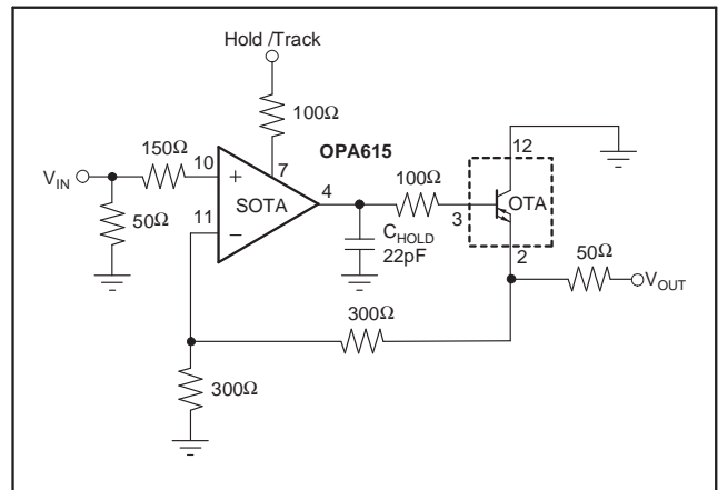
Figure 45. Sample-and-Hold Amplifier
